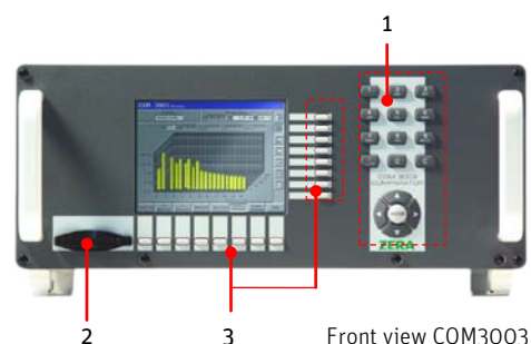
Front view COM3003 Three-phase Comparator
