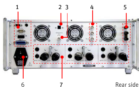
Rear side COM3003
